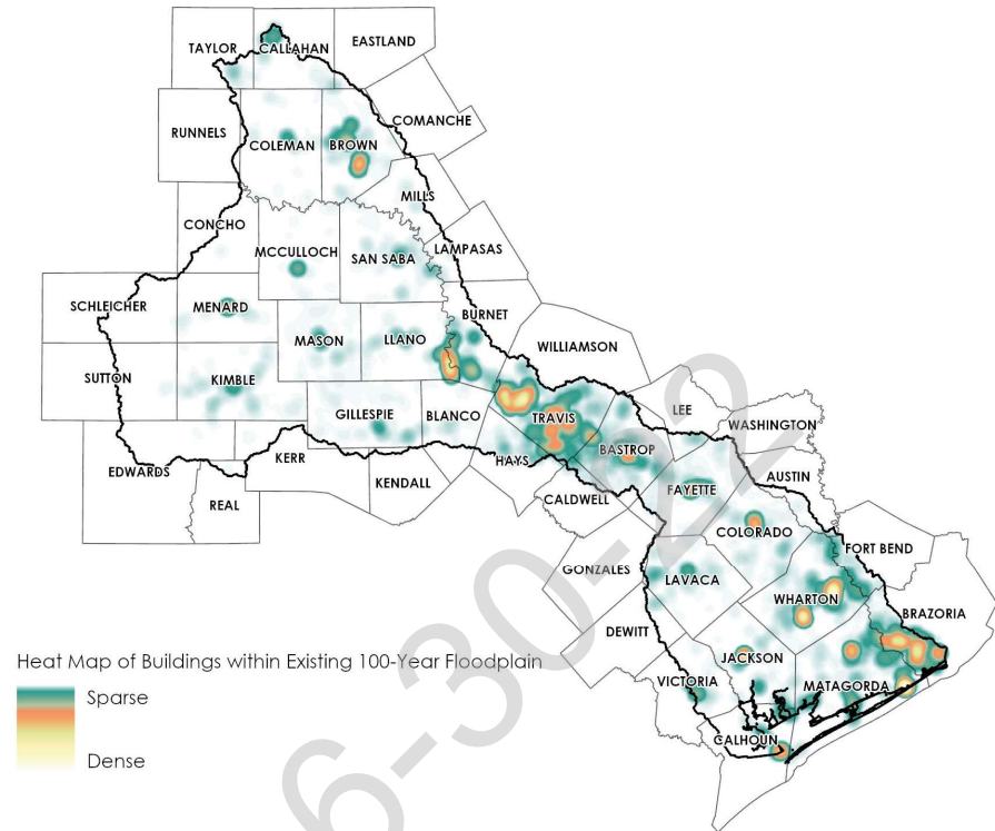
Source: Building Heat map derived from existing condition floodplain in relation to the TWDB building footprints.
